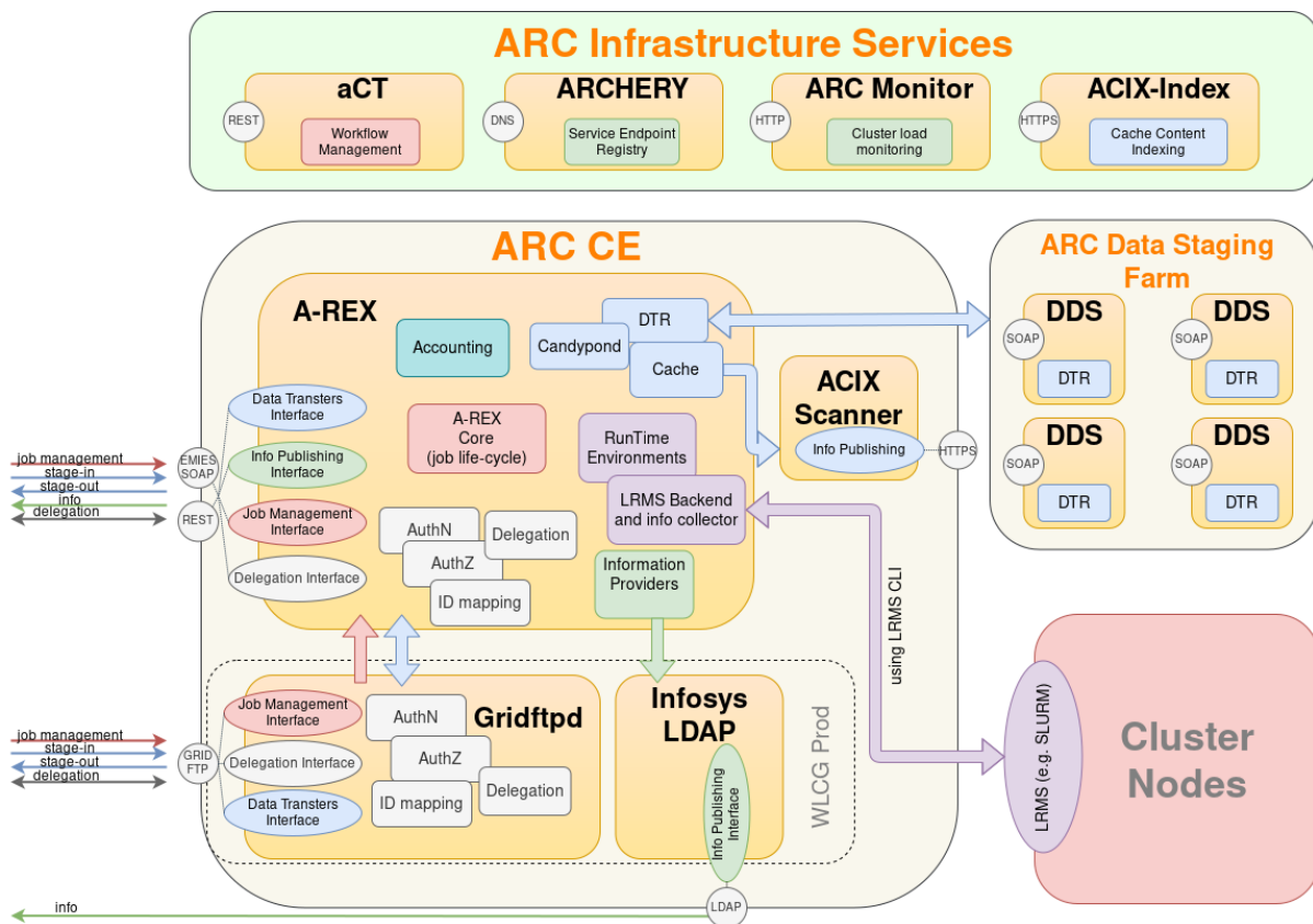
Fig. 1.1: ARC CE: internals, interfaces and the infrastructure ecosystem services around
