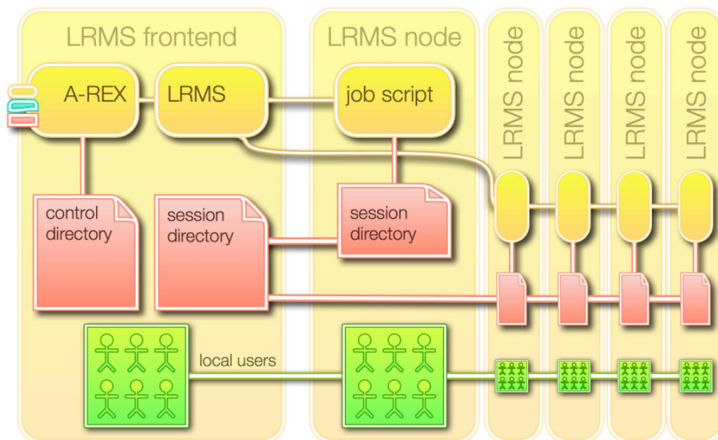
LRMS nodes
