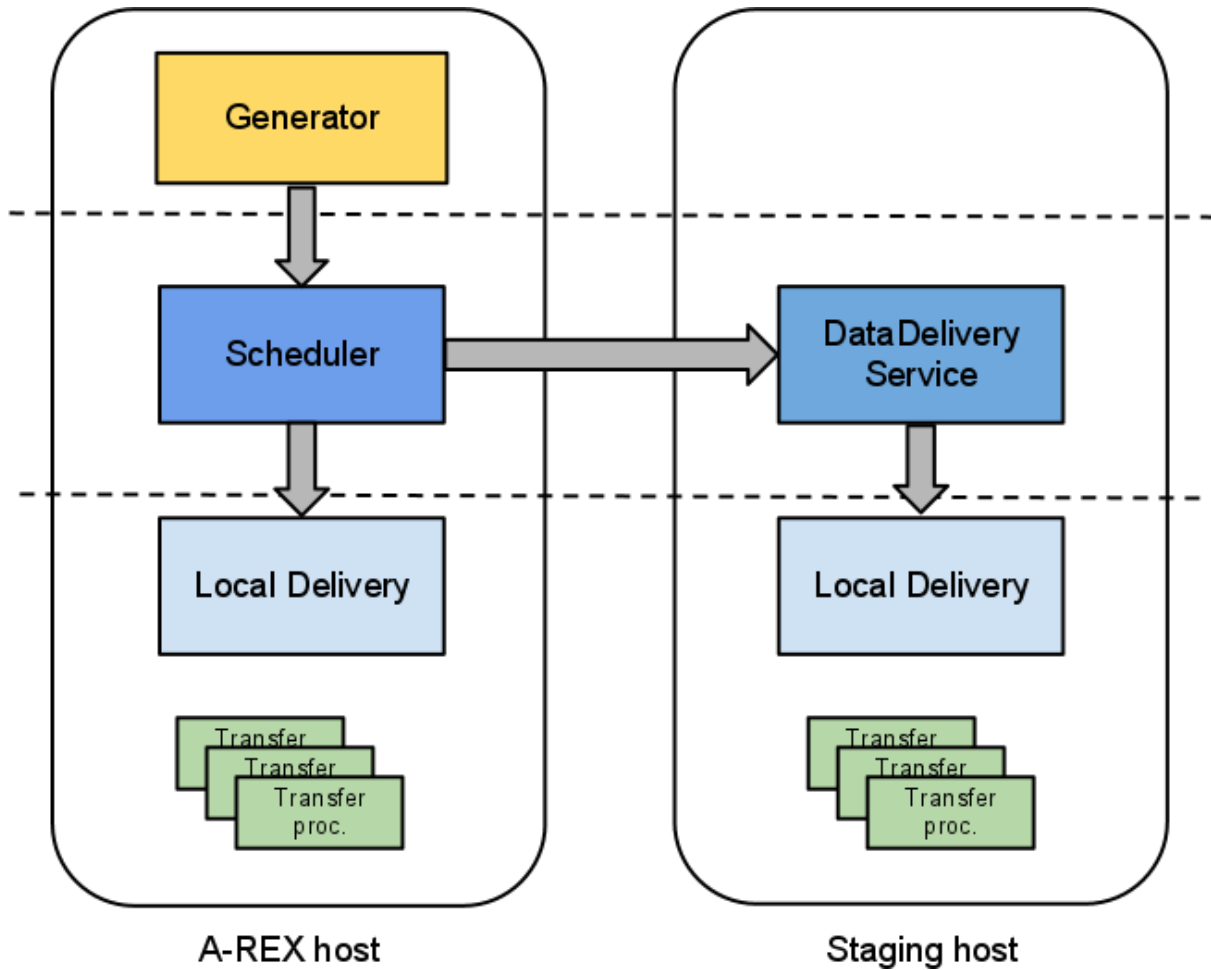
Fig. 5.8: Multi-host datastaging
